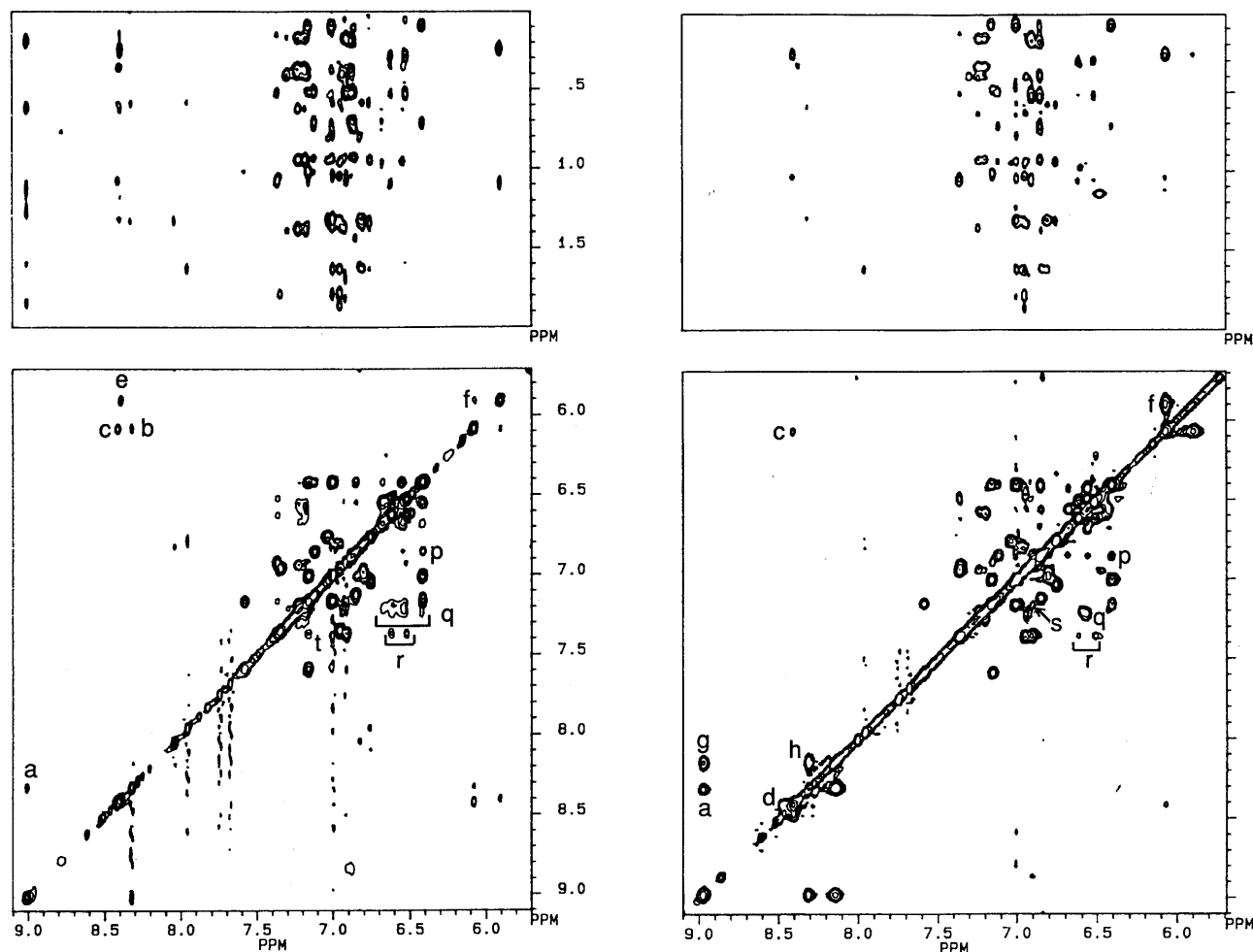
FIGURE 6: NOESY spectrum of R44M+MgAP 5 A (the same sample used for Figure 4B). The cross-peaks a-f and p-t are the same as those for WT+MgAP 5 A explained in Figure 5, except that peak d is obscured by the diagonal and peak s is not resolved.
