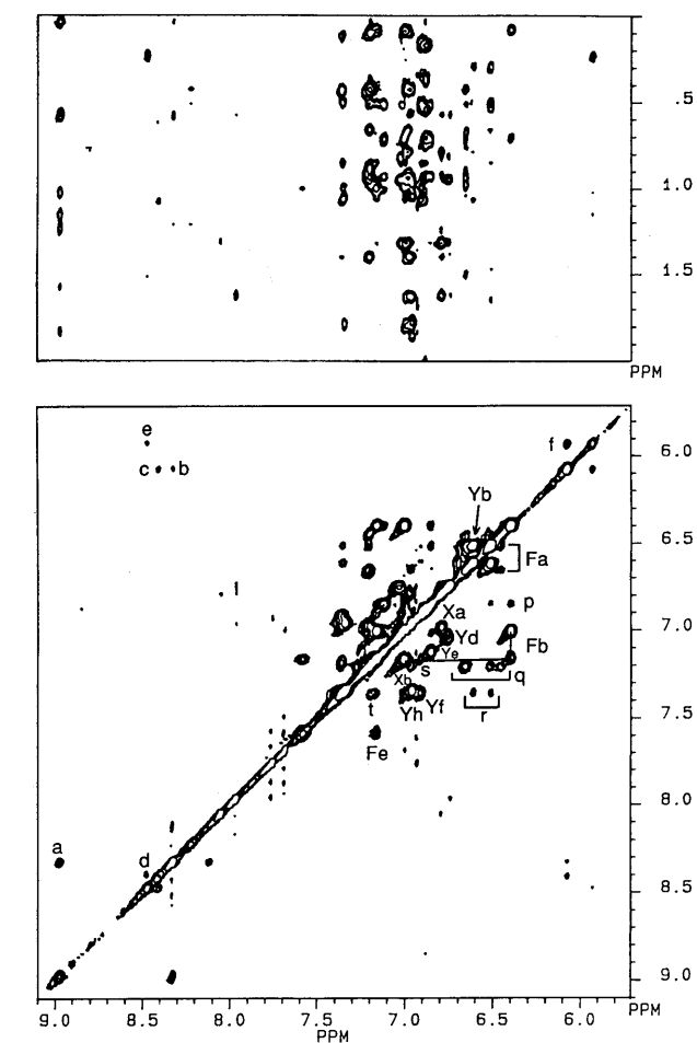
FIGURE 5: NOESY spectrum of WT+MgAP 5 A (the same sample used for Figure 4A). The cross-peaks a–f are due to bound MgAP 5 A: (a) exchange cross-peak between H 2 (I) and H 2 (II); (b) NOE cross-peak between H 2 (II) and H 1 (II); (c) NOE cross-peak between H 8 (II) and H 1 (II); (d) exchange cross-peak between H 8 (I) and H 8 (II); (e) NOE cross-peak between H 8 (I) and H 1 (I); (f) exchange cross-peak between H 1 (I) and H 1 (II). The cross-peaks p–t have been tentatively assigned to interresidue NOE for Fb/Ye, Fa/Xb, Yb/Yf, Fb/Yf, and Fe/Yf, respectively (Yan et al., 1990).
