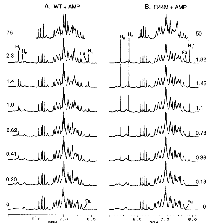
FIGURE 8: Proton NMR titration of WT (A) and R44M (B) with AMP. The starting concentrations of free AK are 1 mM. The ratios [AMP]/[AK] are shown in the figure. Only the spectra in the low ratio range are shown, except that the fully saturated complexes are shown on the top. The labeled peaks H 2 , H 8 , and H 1' are the AMP resonances, whereas Fa is a protein resonance as defined in Table II. The results, but not the spectra, of the WT titration with AMP have been reported in Sanders et al. (1989).
