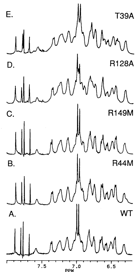
FIGURE 2: One-dimensional proton NMR spectra showing the aromatic regions of WT (A), R44M (B), R149M (C), R128A (D), and T39A (E). The spectra were obtained at pH 7.8, 27 °C, and with Gaussian multiplication (LB = -5, GB = 0.1). The spin systems of WT have been reported in Yan et al. (1990).
